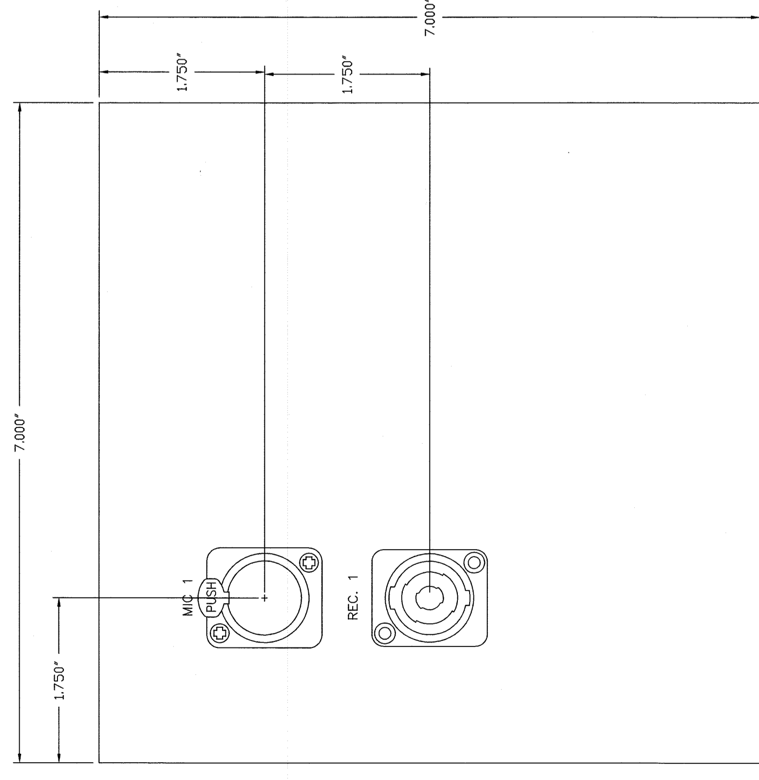
A JUDGE PLATE DETAIL --- MOUNT TO J7 ACTUAL SIZE
