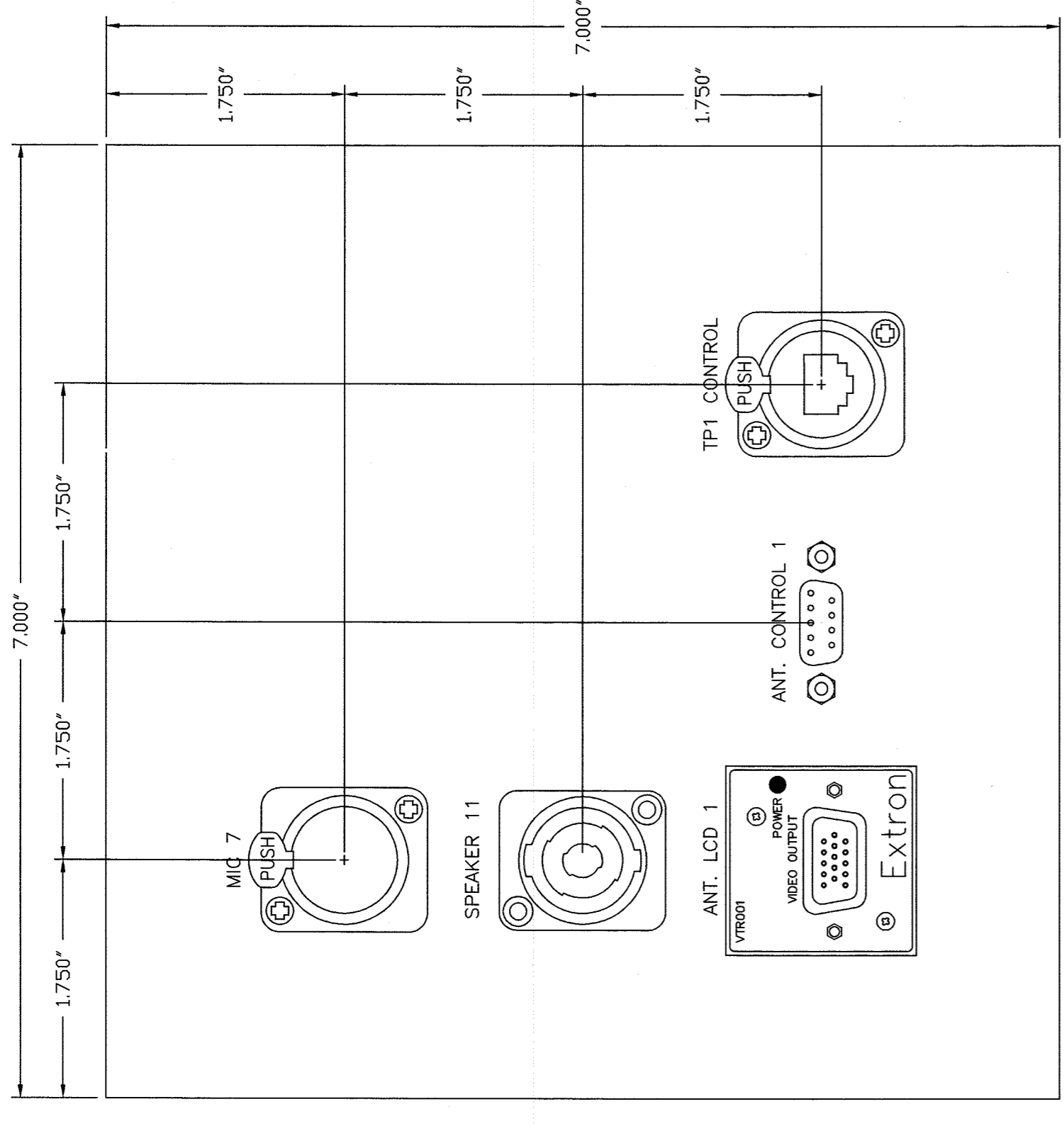
G JUDGE PLATE DETAIL --- MOUNT TO J13 ACTUAL SIZE
