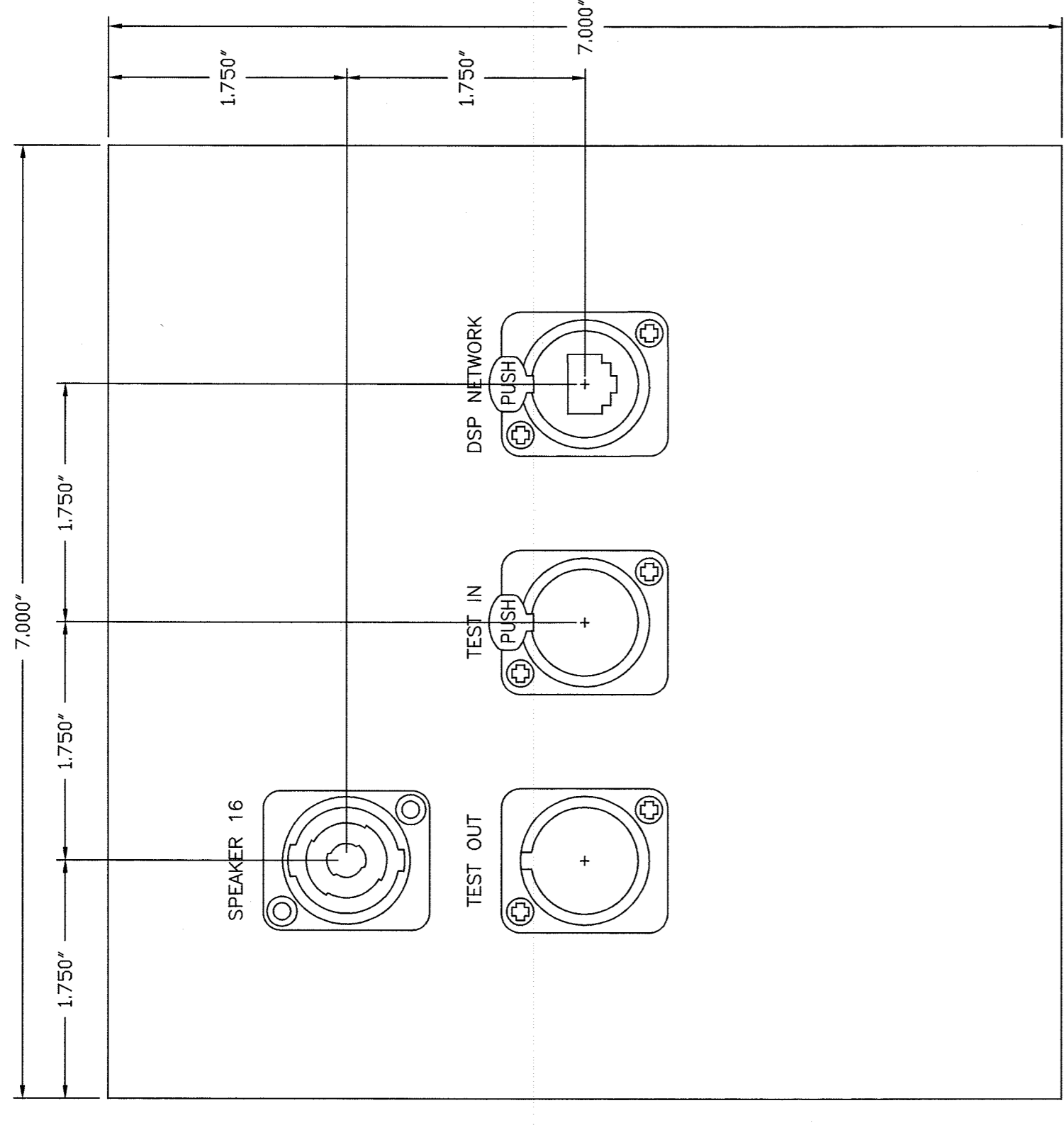
I STENOGRAPHER PLATE DETAIL --- MOUNT TO J12 ACTUAL SIZE
