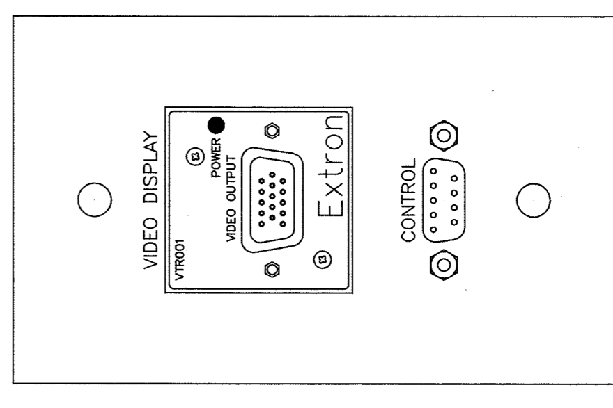
M LCD SCREEN VIDEO FEED PLATE DETAIL --- TYP. 4 MOUNT TO J17, J21, J22, J24 ACTUAL SIZE
