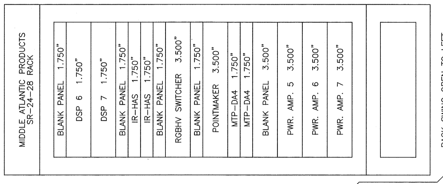
C EQUIPMENT RACK DETAIL ROOM 353 SCALE: 1:500" = 1'-0"
