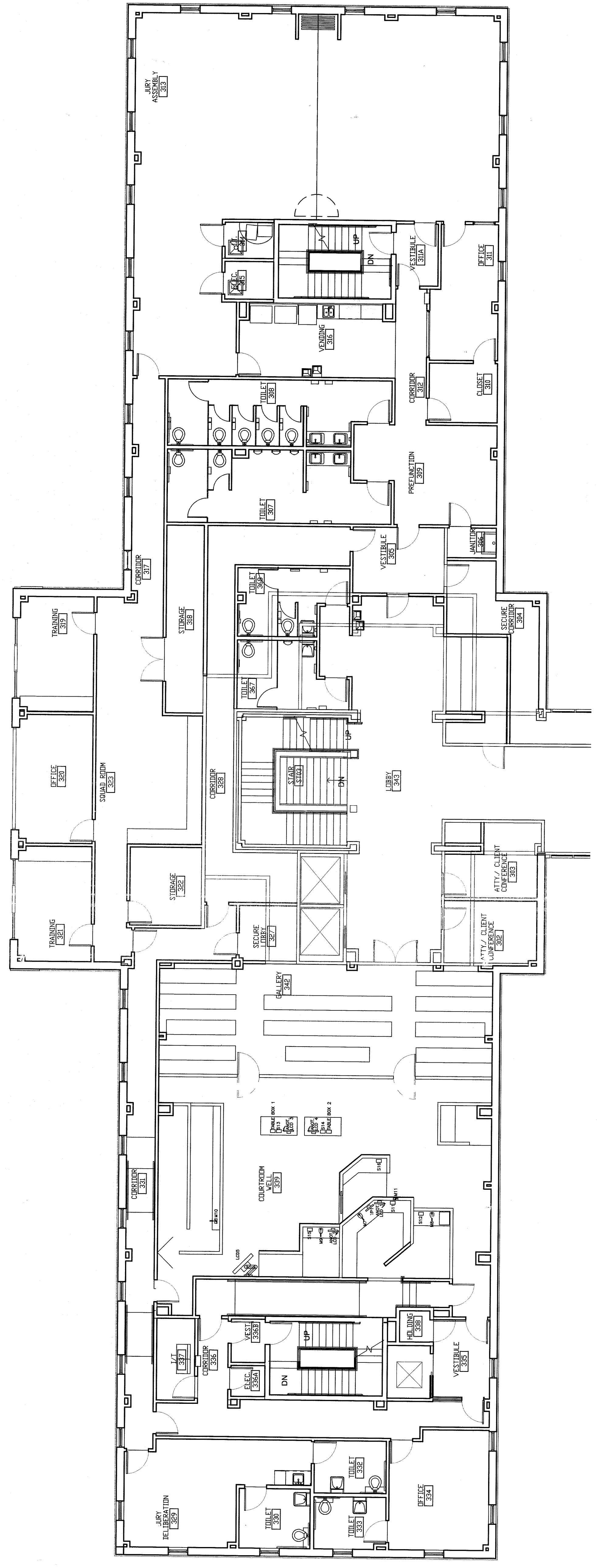
THIRD FLOOR NORTH--FLOOR PLAN--COURTROOM #339 AND JURY ASSEMBLY ROOM #313--EQUIPMENT SCALE: 1/8" = 1'-0"
