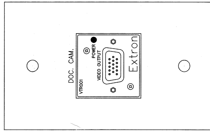
S DOCUMENT CAMERA PLATE DETAIL --- MOUNT J## ACTUAL SIZE
