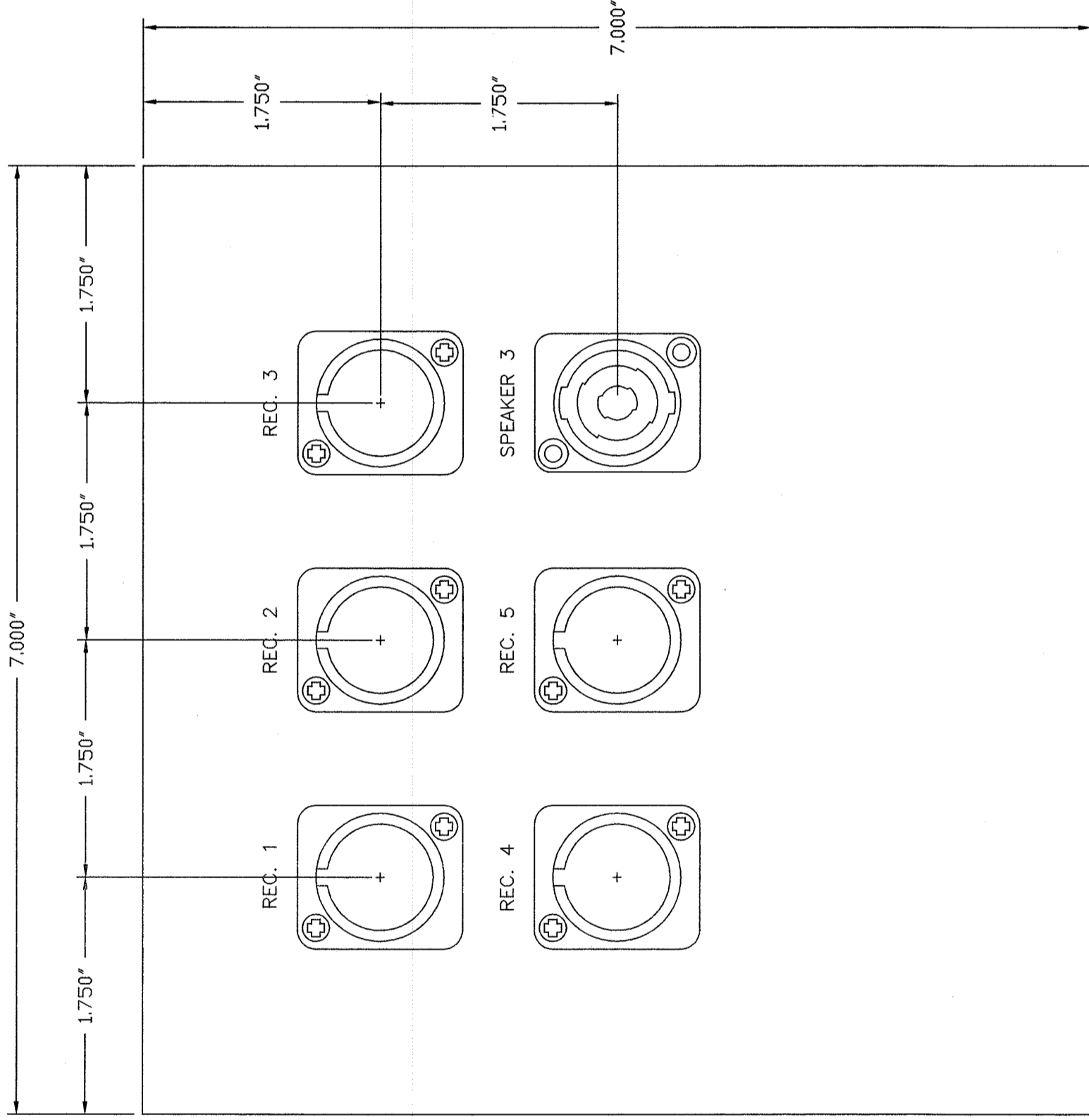
B CLERK PLATE DETAIL --- MOUNT TO J8 ACTUAL SIZE
