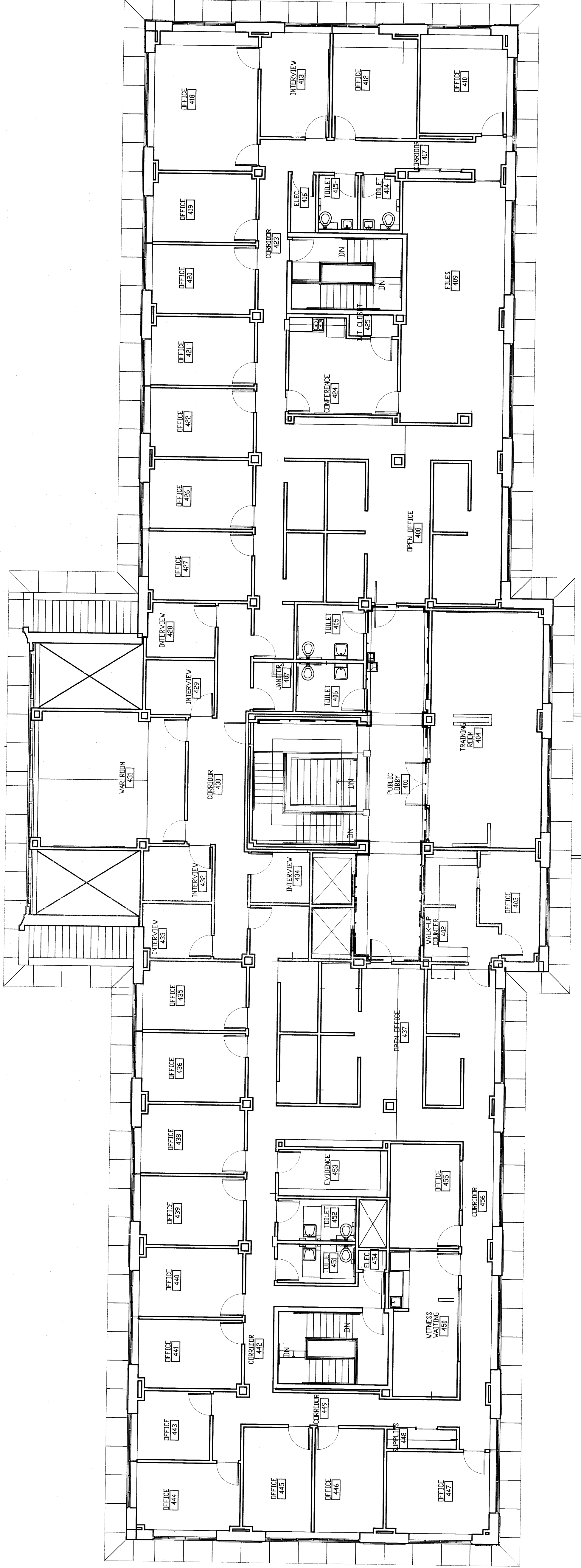
FOURTH FLOOR NORTH--REFLECTED CEILING PLAN--TRAINING ROOM #404--CONDUIT SCALE: 1/8" = 1'-0"
