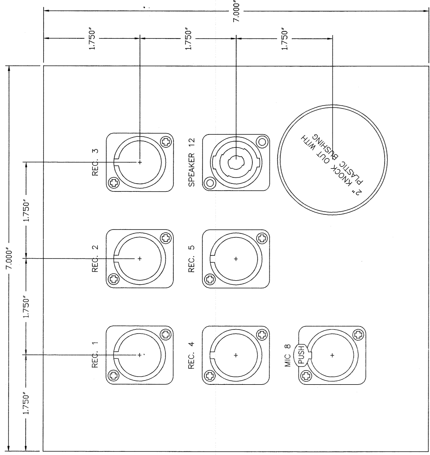
H CLERK PLATE DETAIL --- MOUNT TO J10 ACTUAL SIZE
