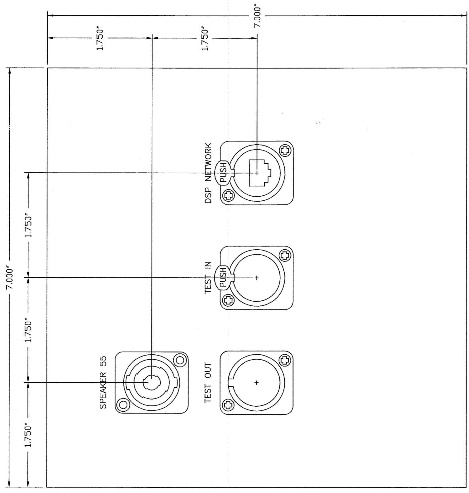
P STENOGRAPHER PLATE DETAIL --- MOUNT TO J42 ACTUAL SIZE
