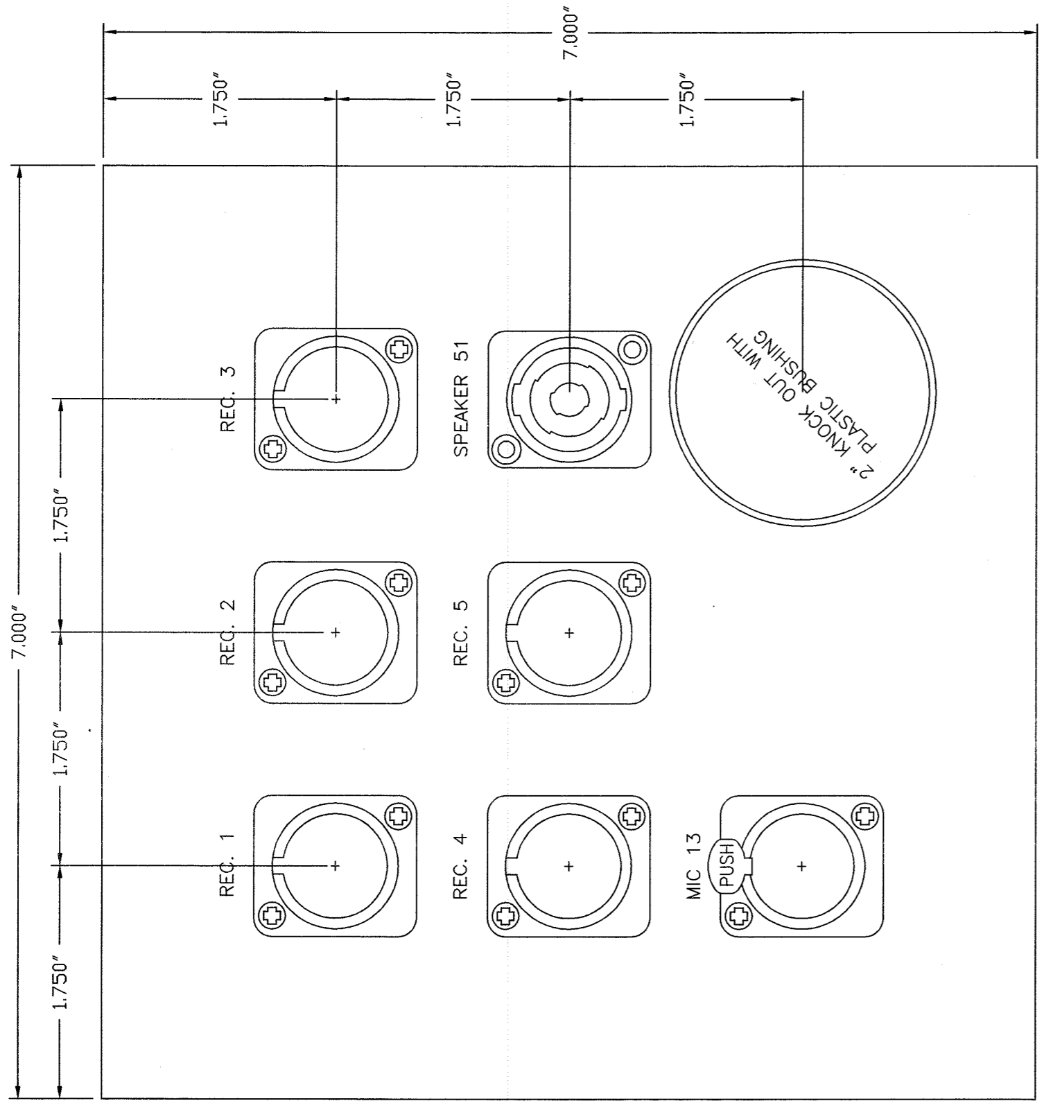
O CLERK PLATE DETAIL --- MOUNT TO J41 ACTUAL SIZE
