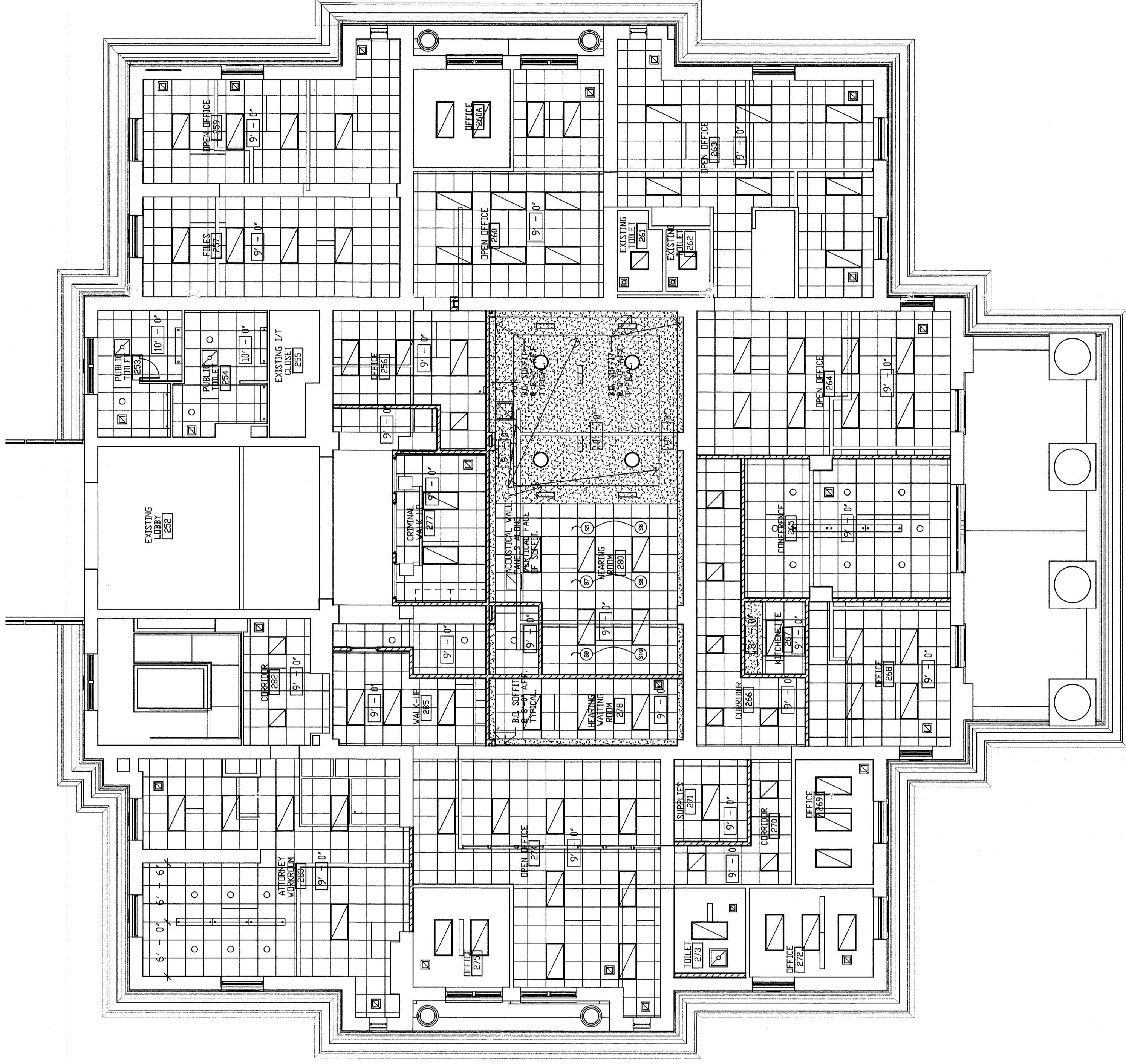
SECOND FLOOR SOUTH--REFLECTED CEILING PLAN--HEARING ROOM #280--EQUIPMENT SCALE: 1/8" = 1'-0"
