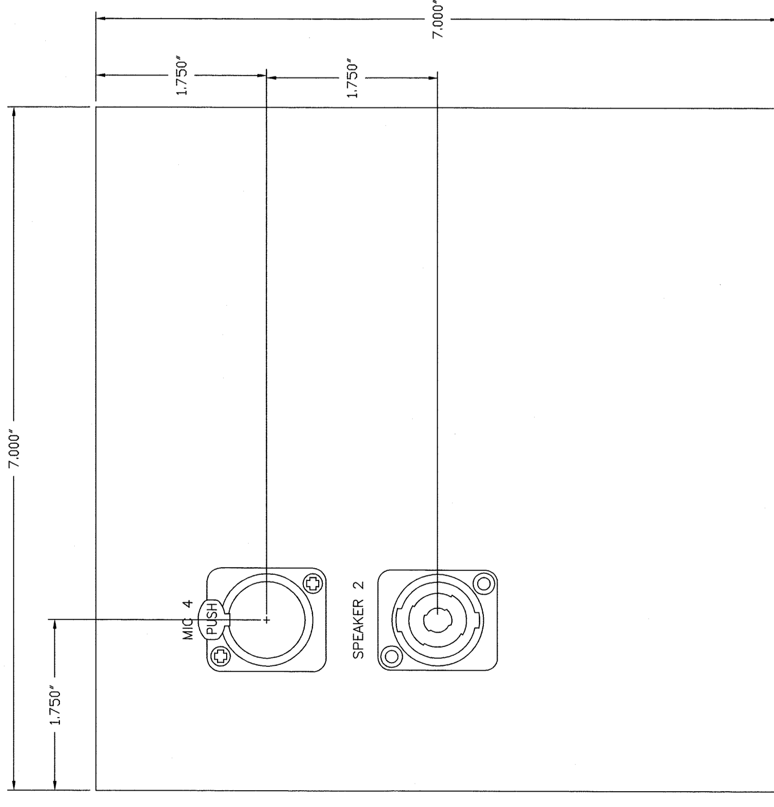
D WITNESS PLATE DETAIL --- MOUNT TO J4 ACTUAL SIZE
