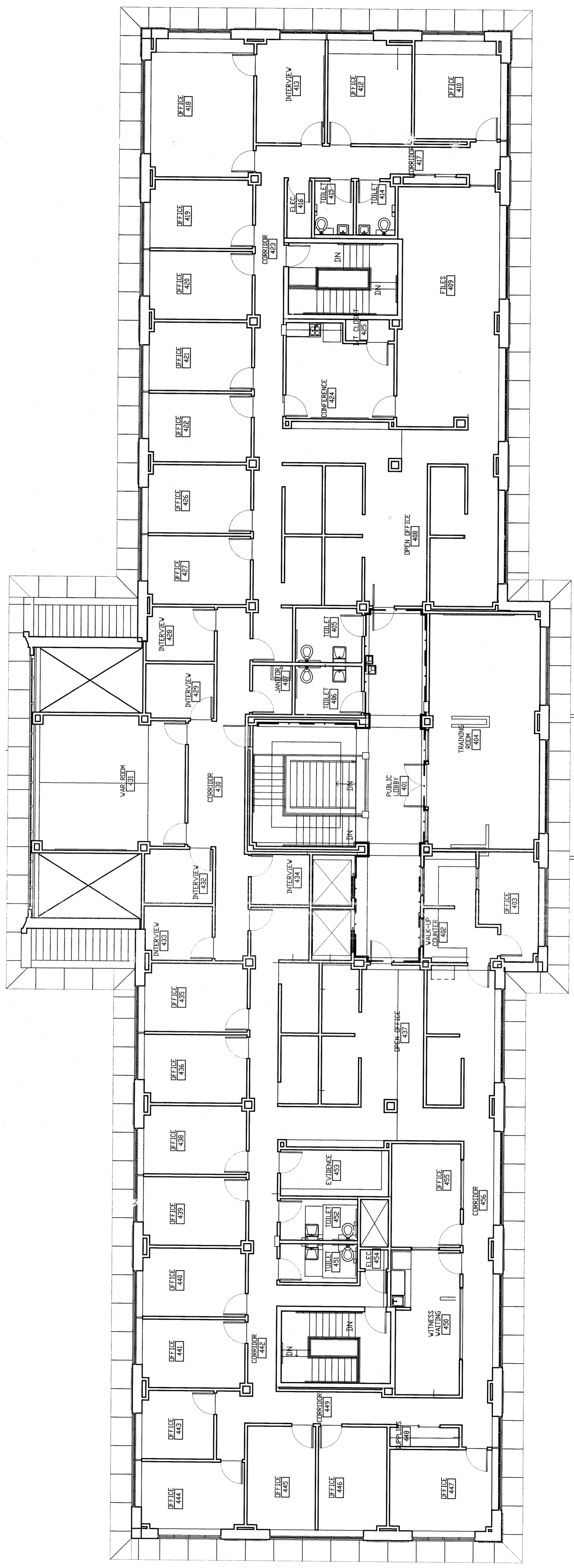
FOURTH FLOOR NORTH--REFLECTED CEILING PLAN--TRAINING ROOM #404--EQUIPMENT SCALE: 1/8" = 1'-0"
