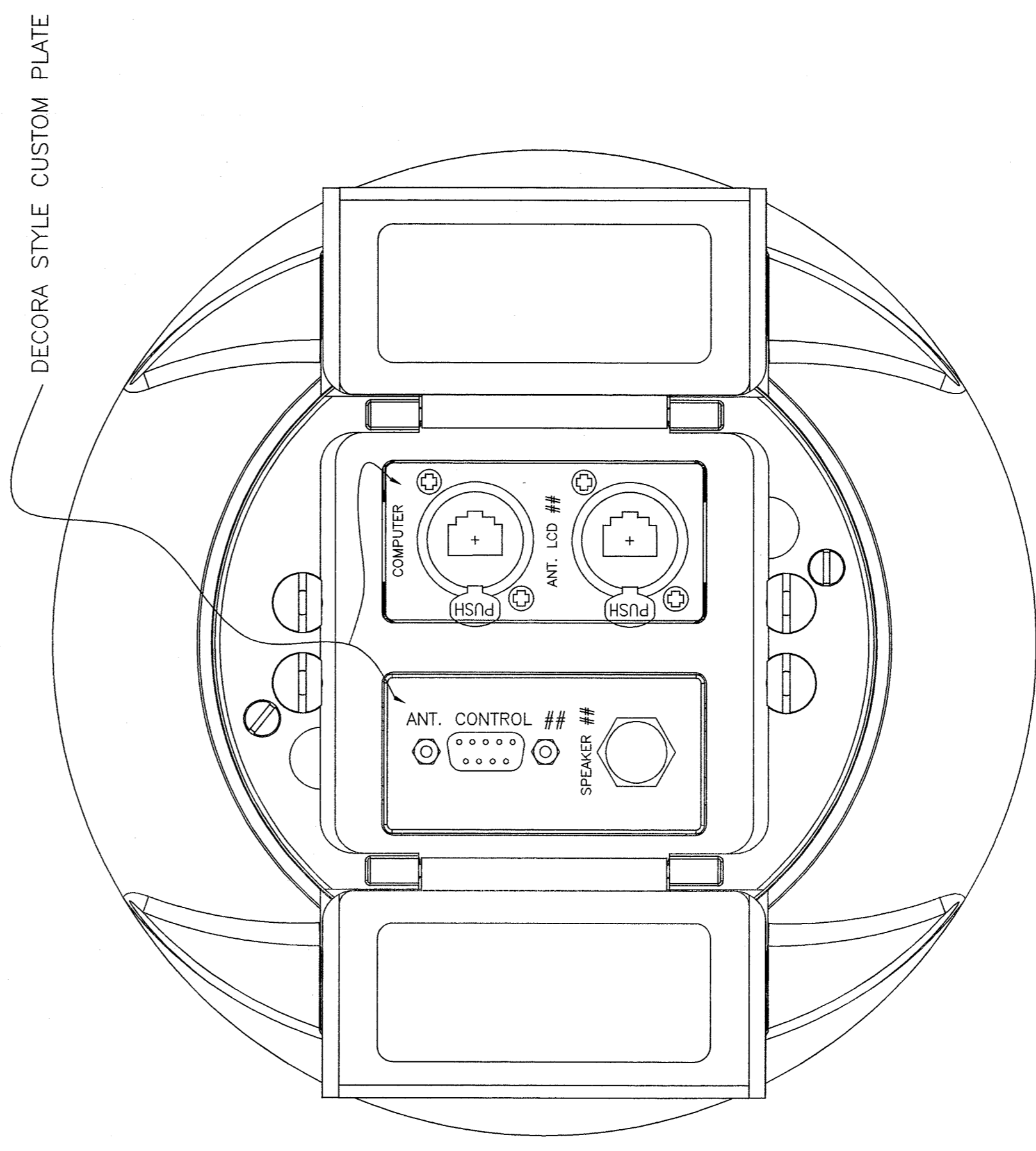
K PROSECUTING / DEFENCE POKE THROUGH FLOOR BOX --- J15 / J16 SPEAKER 13, ANT. 3 FOR PROSECUTING AND SPEAKER 14, ANT. 4 FOR DEFENCE ACTUAL SIZE
