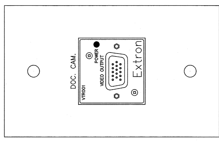
L DOCUMENT CAMERA PLATE DETAIL --- MOUNT TO J## ACTUAL SIZE
