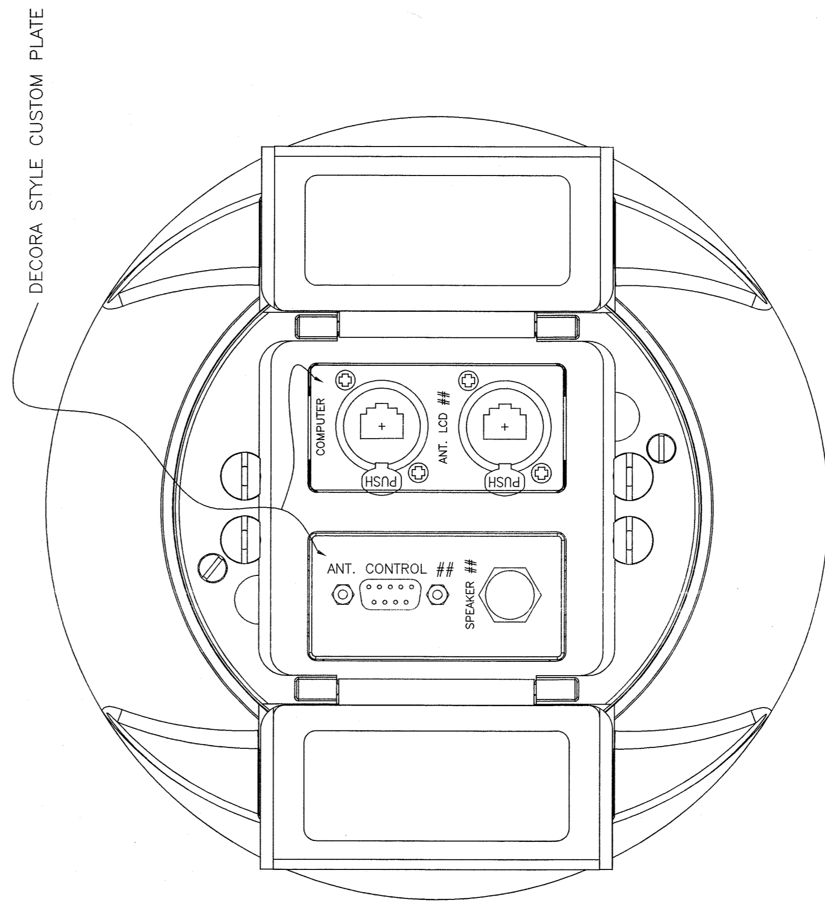
R PROSECUTING / DEFENCE POKE THROUGH FLOOR BOX --- J451 / J46 SPEAKER 52, ANT. 7 FOR PROSECUTING AND SPEAKER 53, ANT. 8 FOR DEFENCE ACTUAL SIZE
