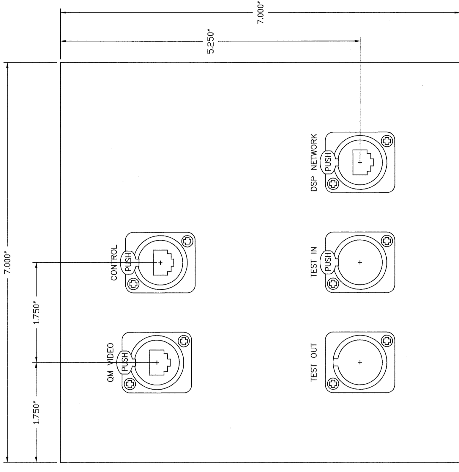
C VIDEO CART WALL PLATE DETAIL --- MOUNT TO J1 / J30 / J31 / J60 ACTUAL SIZE
