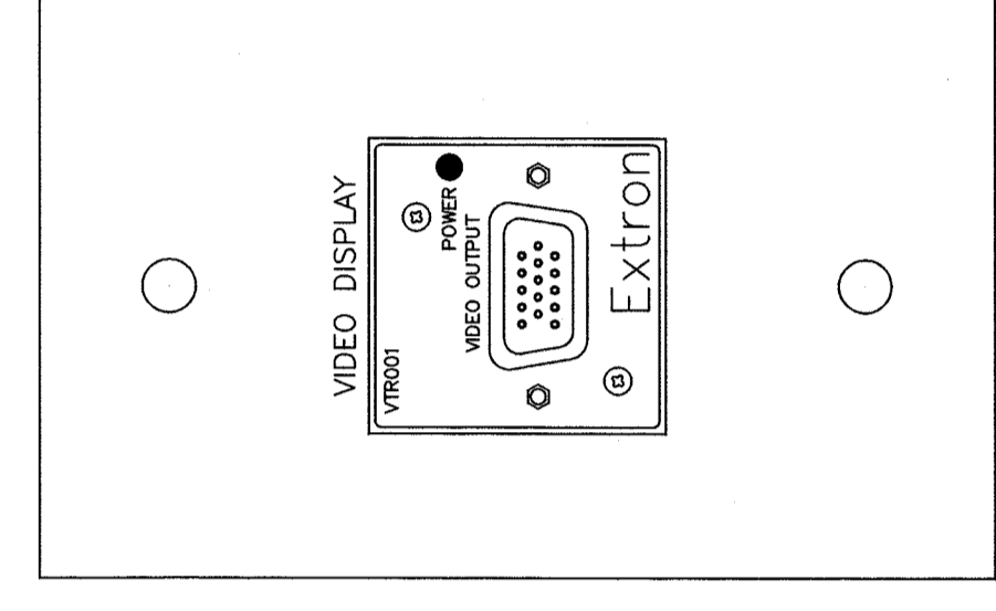
F LCD SCREEN VIDEO FEED PLATE DETAIL --- MOUNT U2 ACTUAL SIZE
