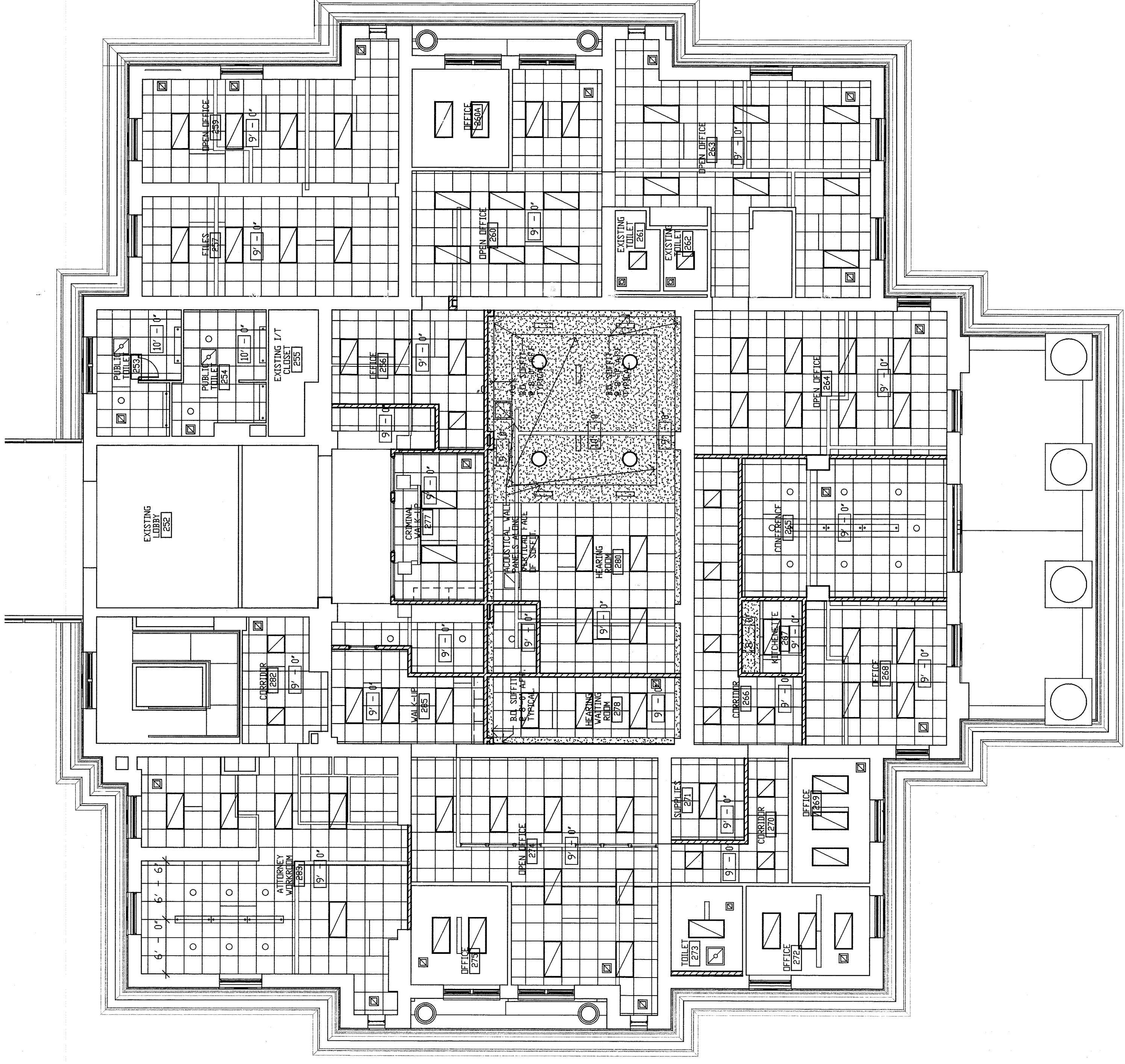
SECOND FLOOR SOUTH--REFLECTED CEILING PLAN--HEARING ROOM #280--CONDUIT SCALE: 1/8" = 1'-0"
